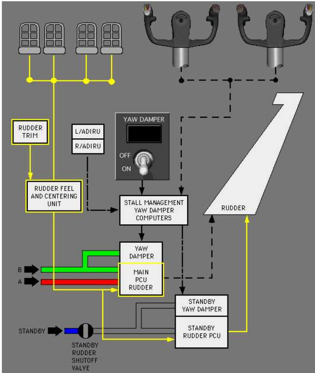
Yaw Control
