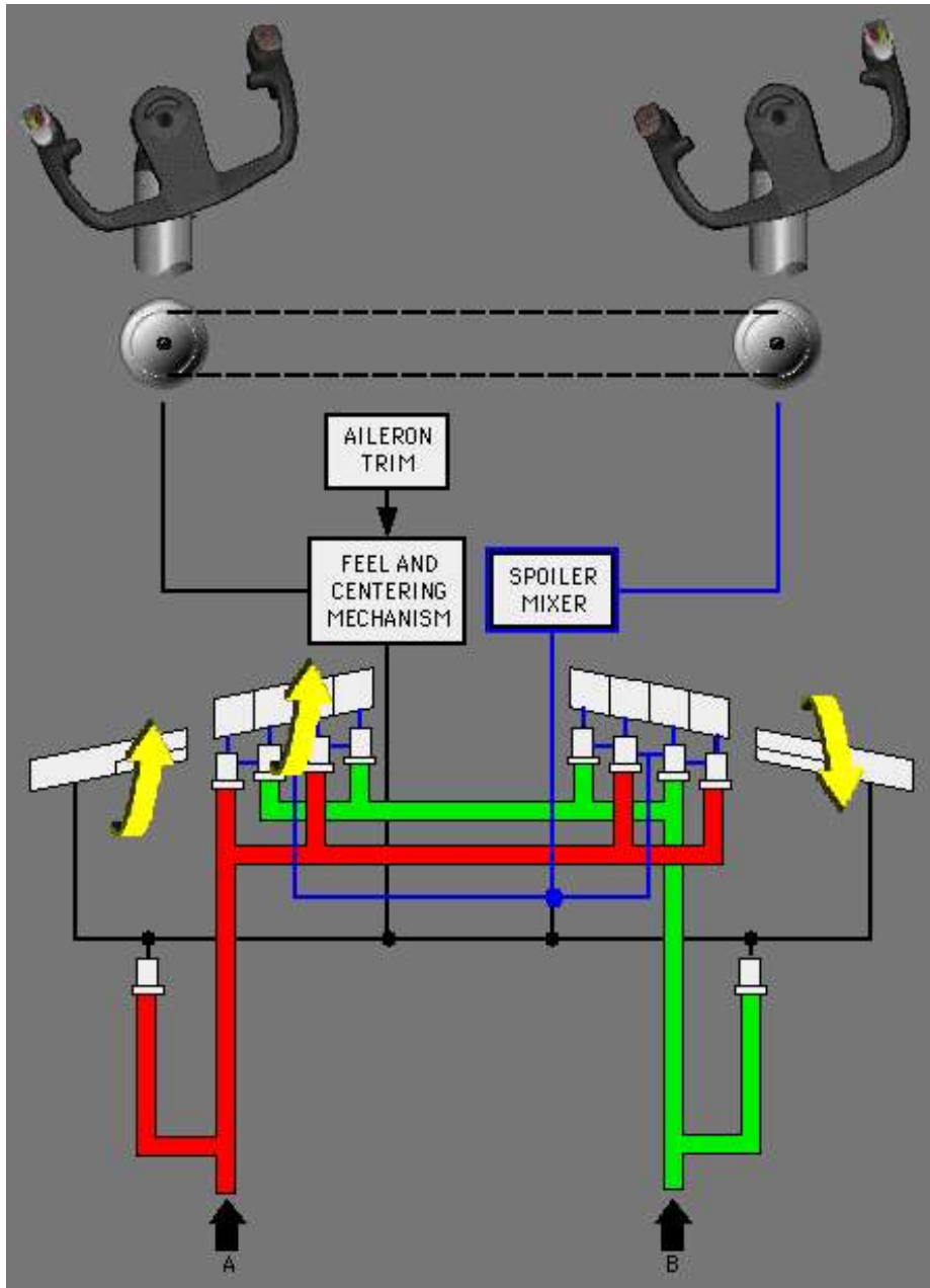
Roll Control
