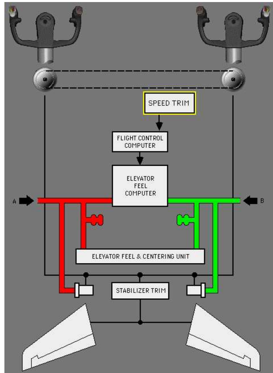
Pitch Control
